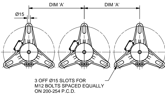
3 PHASE MOUNTING PLAN MINIMUM PHASE CENTRES (mm)
